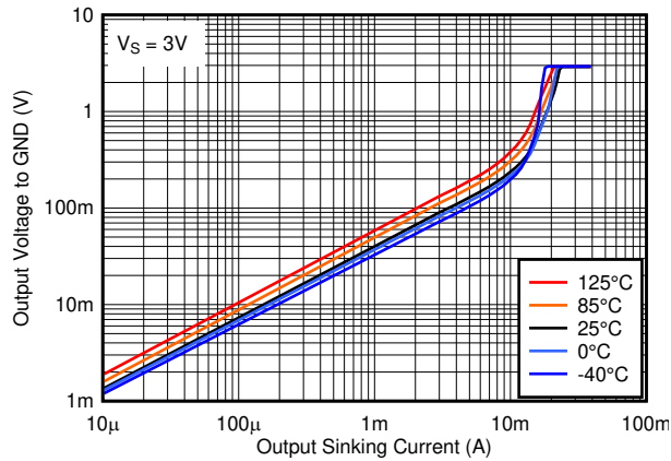
Figure 3-25. Output Low Voltage vs. Output Sinking Current at 3V
