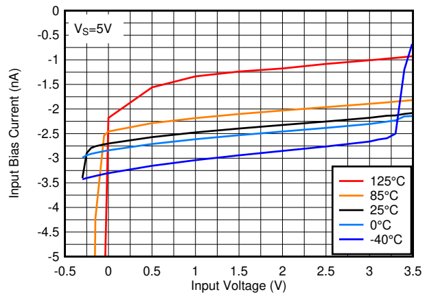
Figure 3-22. Input Bias Current vs. Input Voltage at 5V
