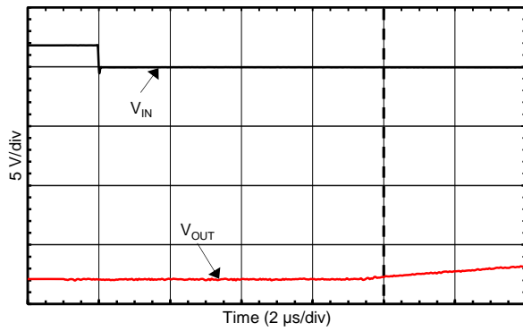
Figure 25. Negative Overload Recovery
