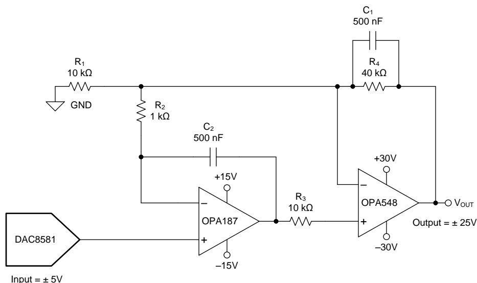
Figure 46. Programmable Power Supply
