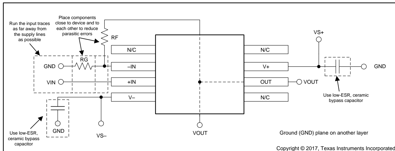
Figure 48. Layout Example
