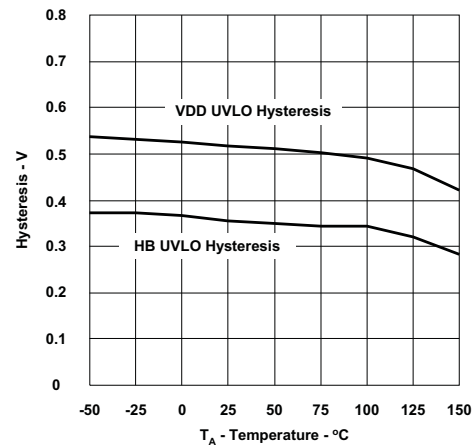
Figure 13. Undervoltage Lockout Threshold Hysteresis vs Temperature
