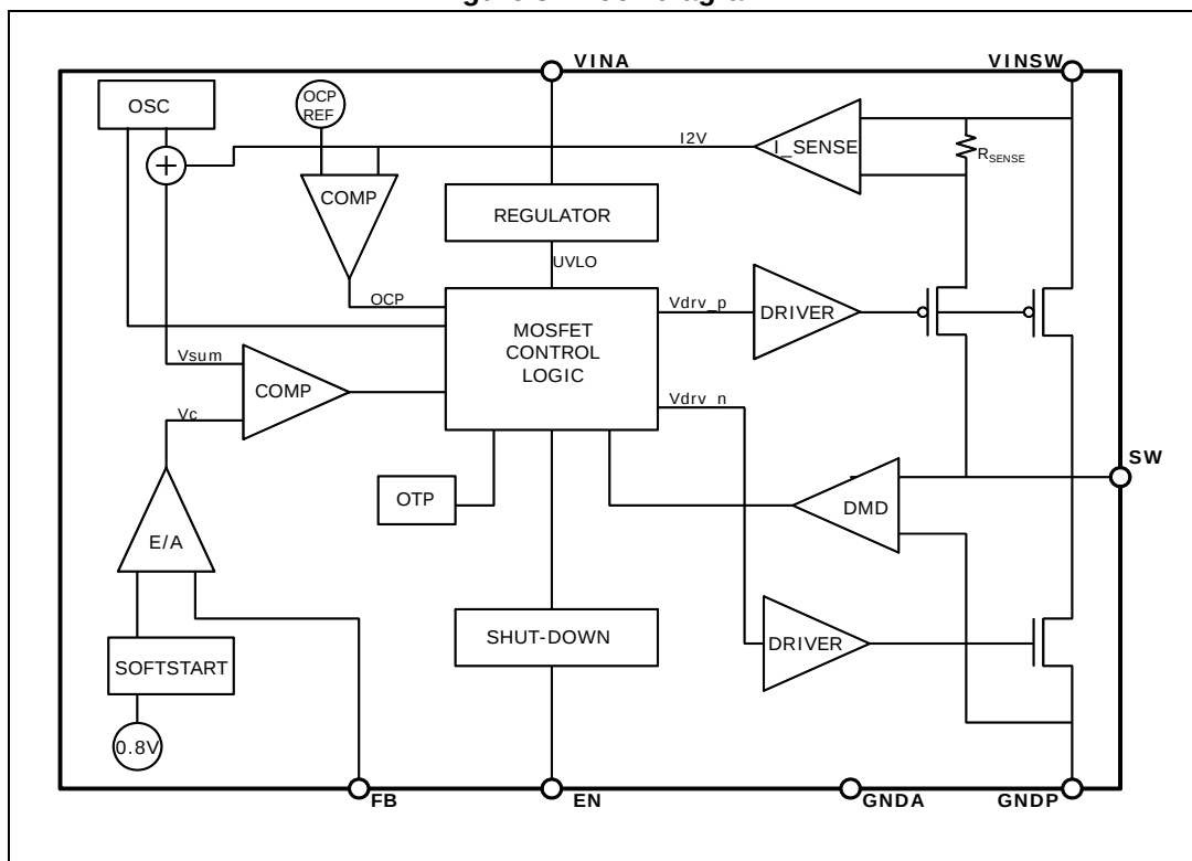
Figure 3. Block diagram
