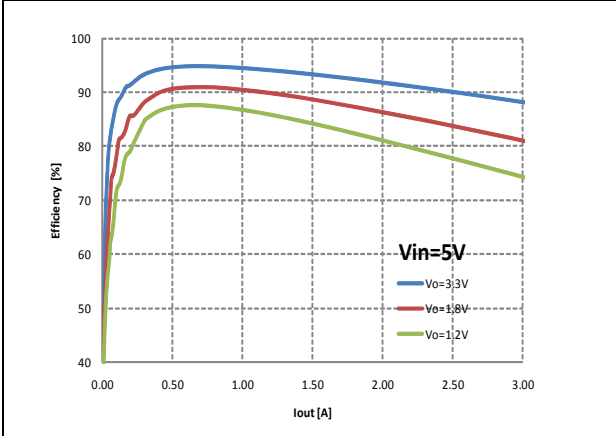
Figure 15. Efficiency vs. I_{OUT}
