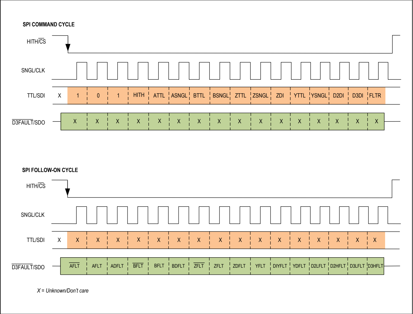
Figure 9. Change Configuration with Detailed Fault Readback SPI Command
