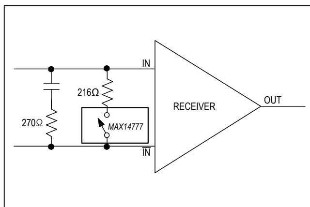
Figure 12. Sample Termination Scheme for HTL, RS-422, and TTL modes
