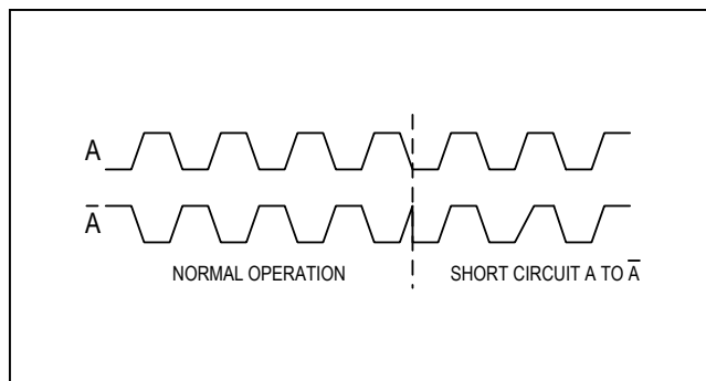
Figure 7. Short Circuit Detection
