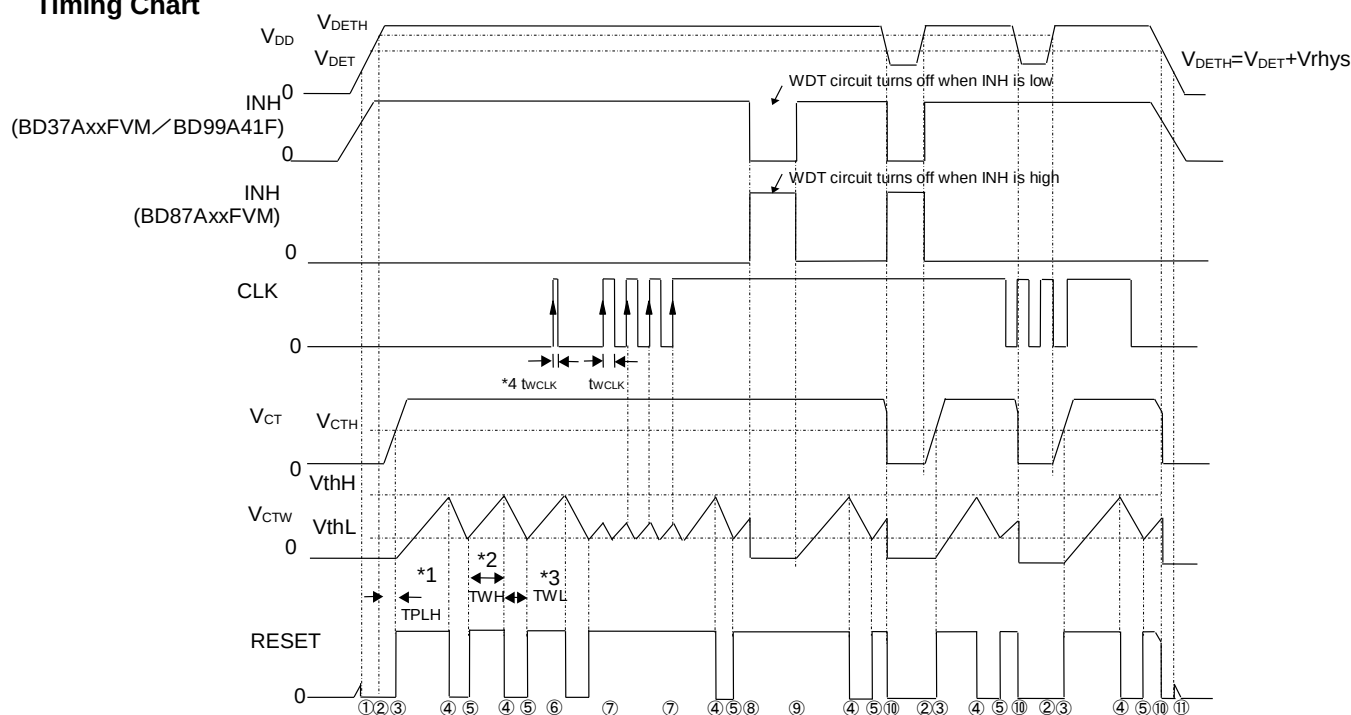
Figure 15. Timing Chart
