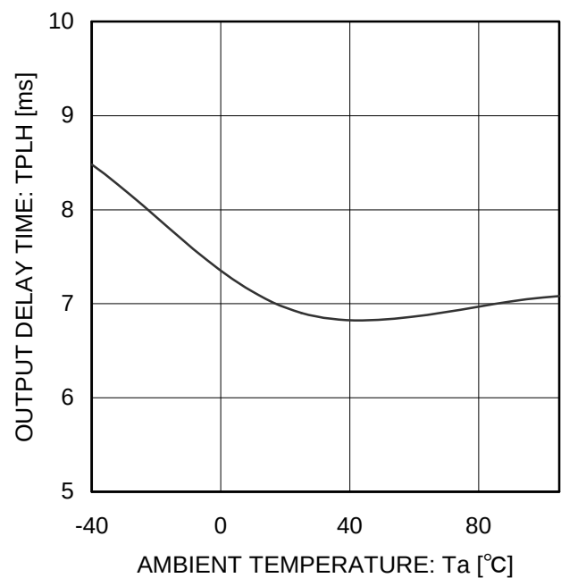
Figure 13. RESET Transmission Delay Time vs Temperature
