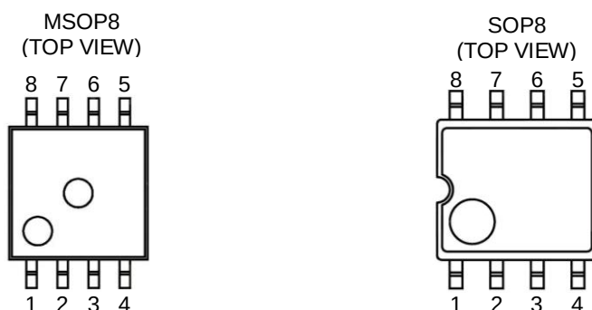
Figure 1. Pin Configurations
