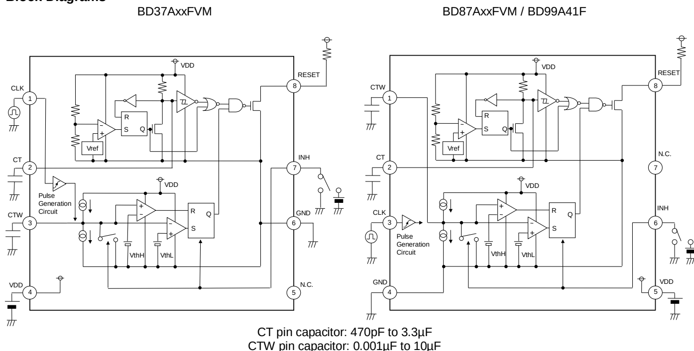
Figure 2. Block Diagrams
