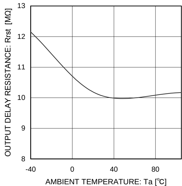
Figure 12. CT Pin Circuit Resistance vs Temperature
