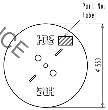
Style and dimension of reel
