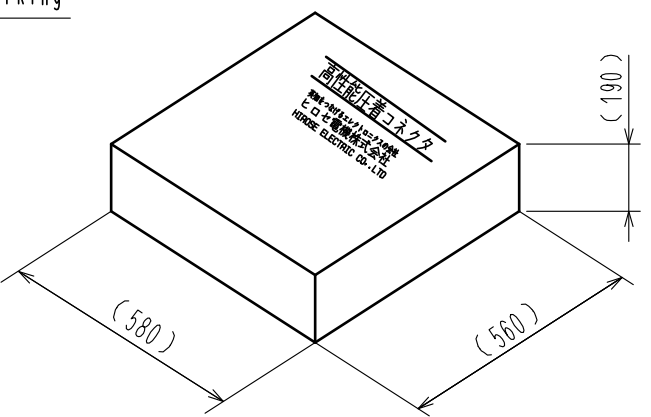
2 Style and dimension of box
