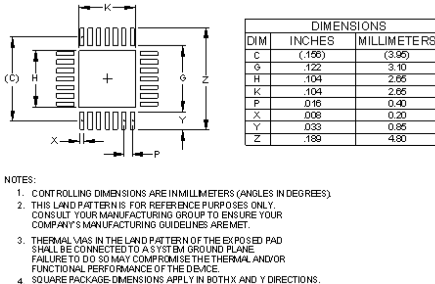
Figure 59 Land Pattern
