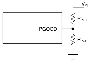
Figure 20. PGOOD Resistor Divider
