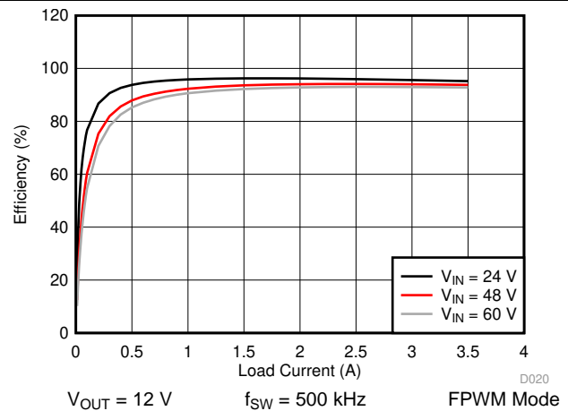
Figure 32. LM76003-Q1 Efficiency
