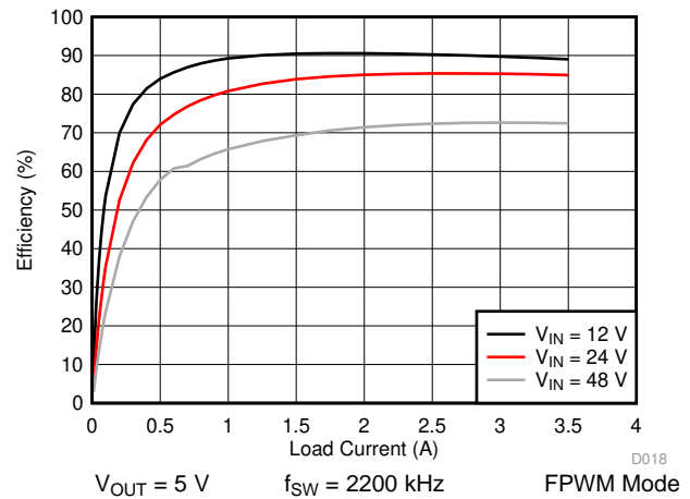
Figure 30. LM76003-Q1 Efficiency
