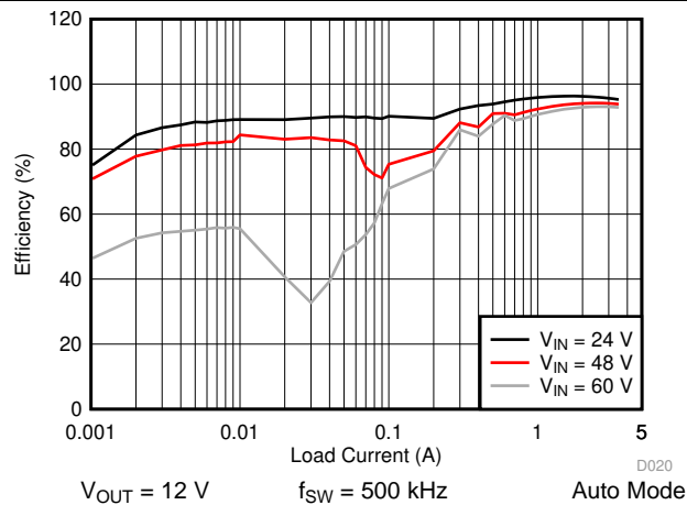
Figure 31. LM76003-Q1 Efficiency
