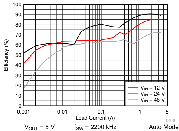
Figure 29. LM76003-Q1 Efficiency
