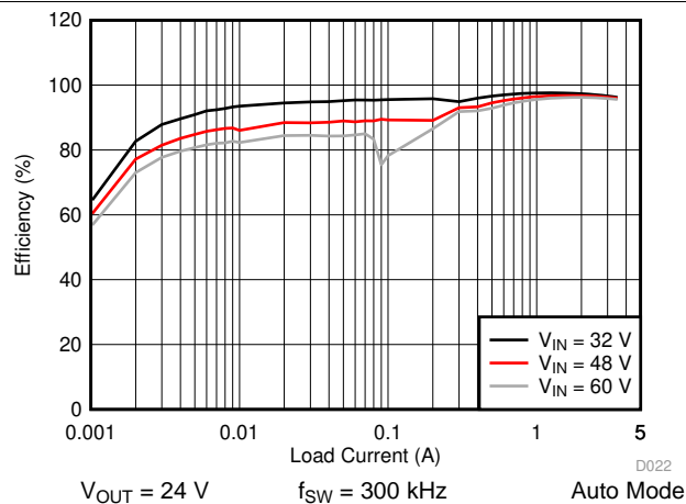
Figure 33. LM76003-Q1 Efficiency
