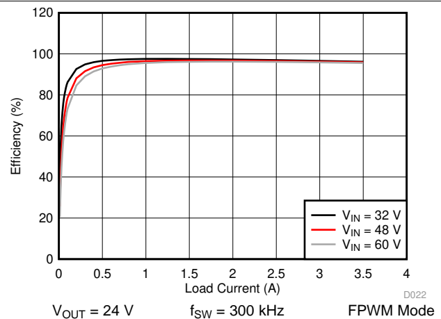
Figure 34. LM76003-Q1 Efficiency
