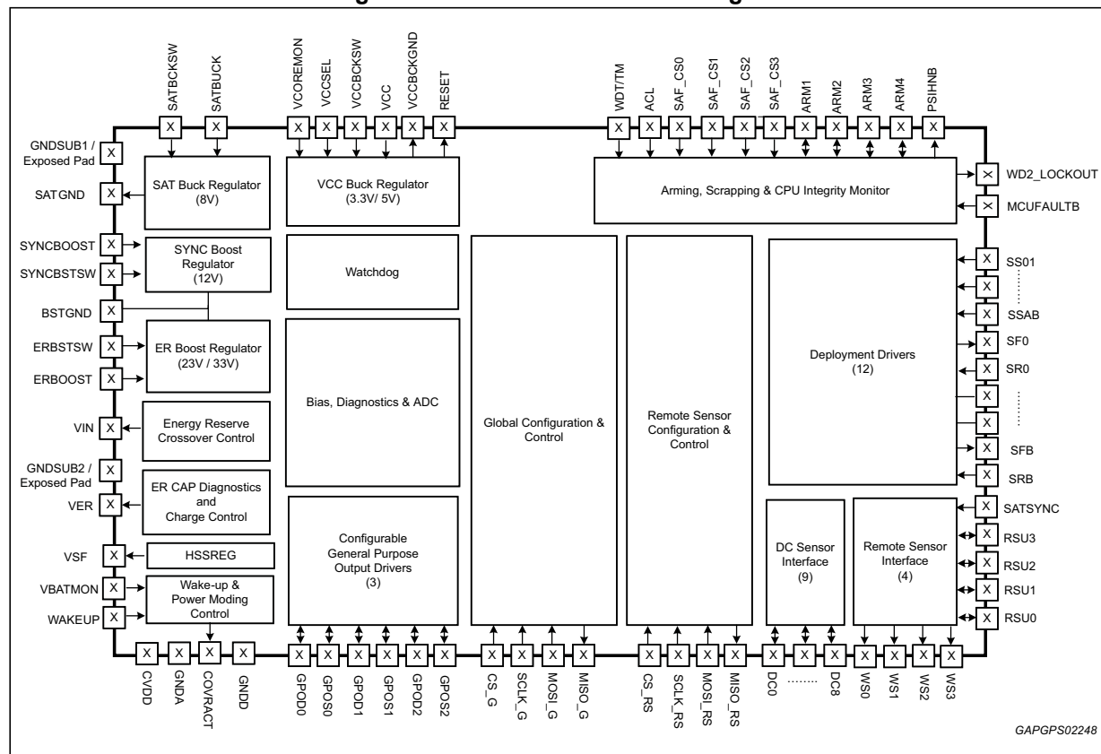
Figure 2. Device function block diagram
