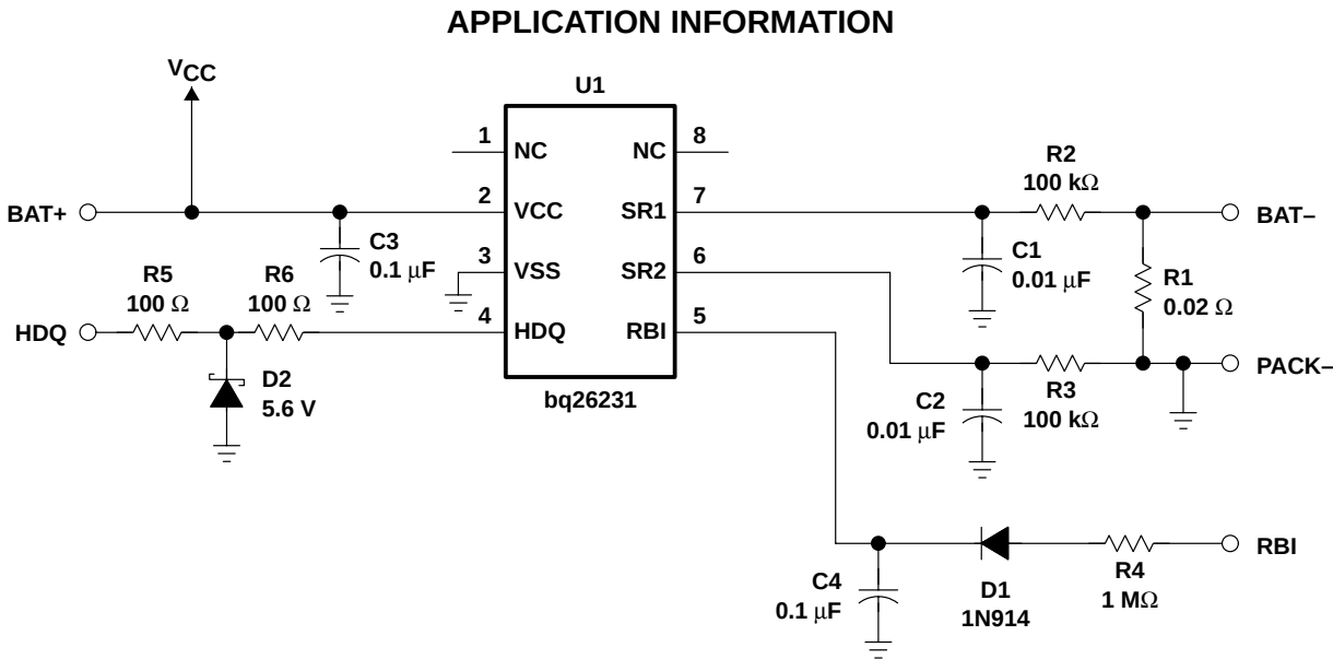
Figure 2. Typical Application
