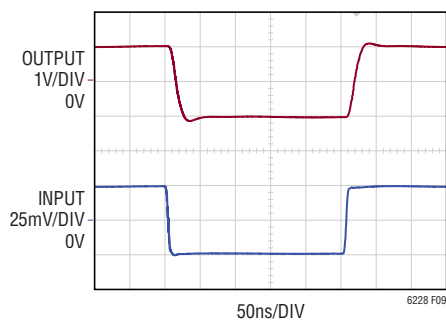
Figure 9. Transient Response
