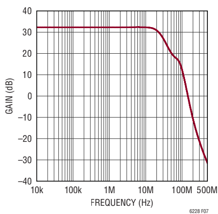
Figure 7. Instrumentation Amplifier Frequency Response
