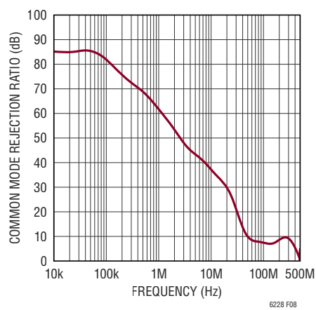
Figure 8. Instrumentation Amplifier CMRR
