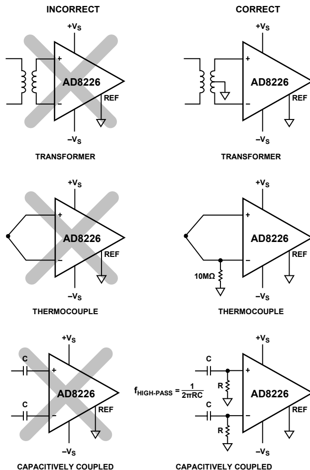
Figure 62. Creating an I_{\text{BIAS}} Path
