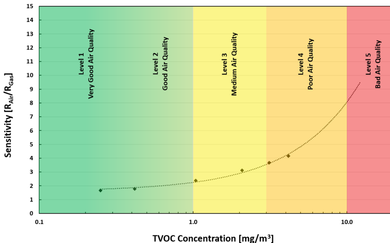
Figure 3. Typical ZMOD4410 Response to Levels of TVOC Described by the UBA using an EPA Standard Mixture
