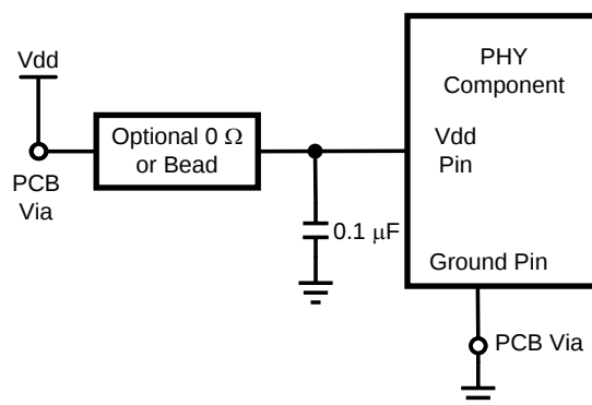
Figure 7-1. V_{DD} Bypass Layout
