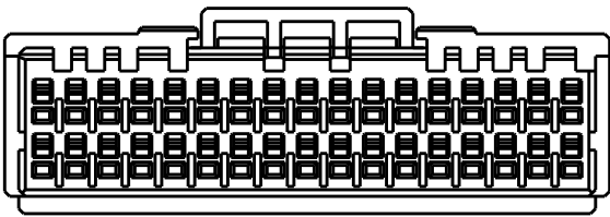
34POS(X-KEY): I-2333134-7
