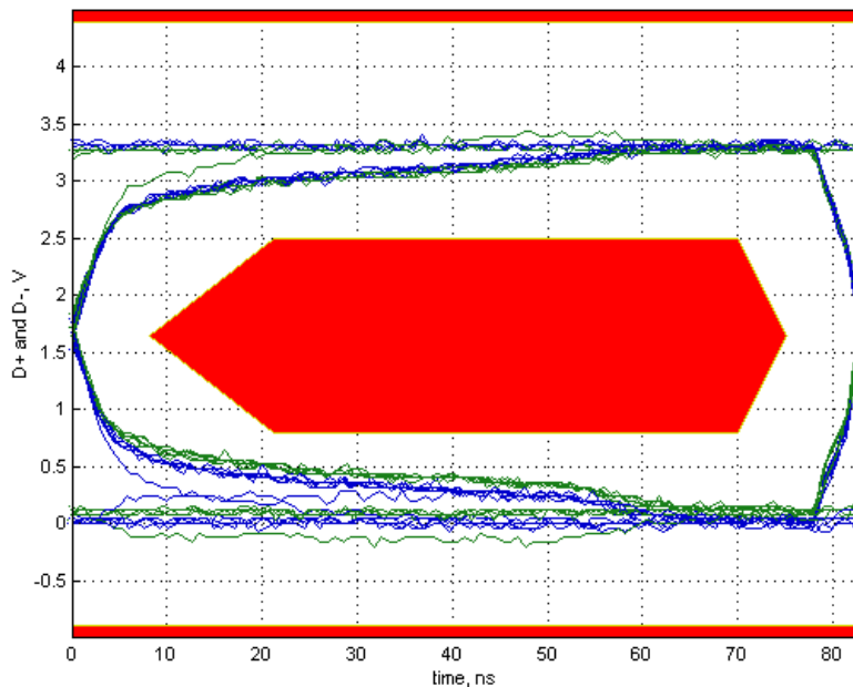
Figure 11. Full Speed Signal Quality Eye Diagram Test (NLAS7222A with V_{CC} = 3.6 V)
