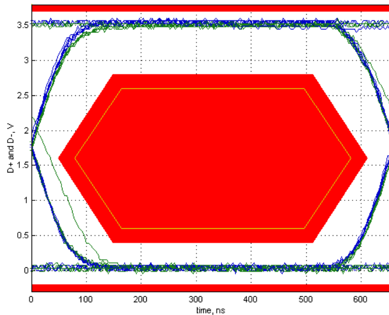
Figure 10. Low Speed Signal Quality Eye Diagram Test (NLAS7222A with V_{CC} = 3.6 V)
