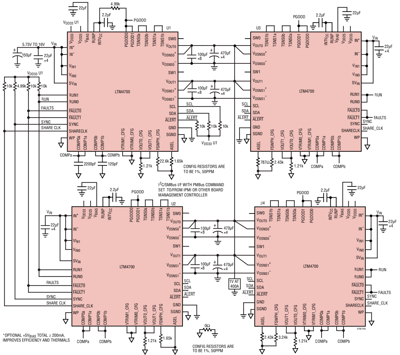
Figure 50. 8-Phase Operation with Four LTM4700 Producing 1V at 400A. Power System Management Features Accessible Through LTM4700 Over 2-Wire I²C/SMBus/PMBus Serial Interface
