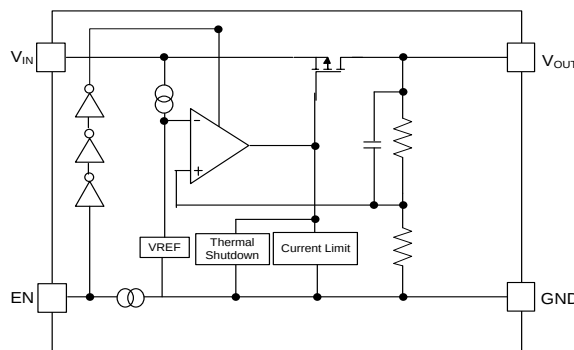
AP7343 (Without Discharge)
