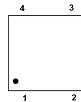
X2-DFN1010-4 (Type B)
