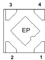
X2-DFN1010-4 (Type B)
