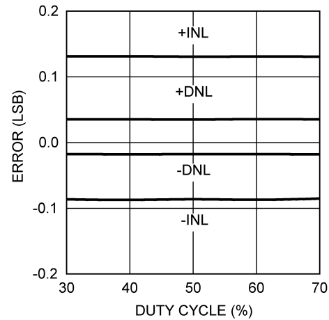
Figure 12. INL/DNL vs Clock Duty Cycle at V_A = 5 V
