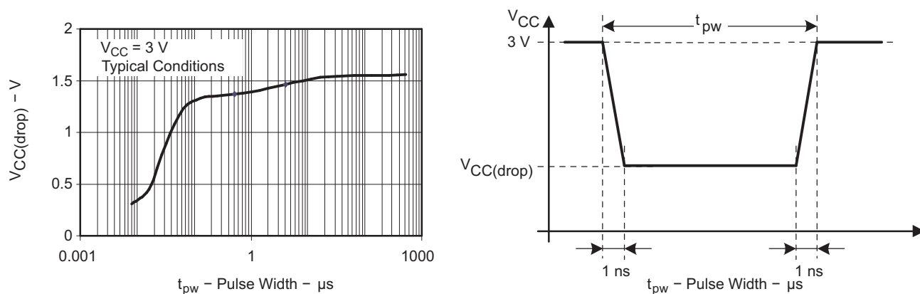
Figure 10. V_{CC(drop)} Level With a Square Voltage Drop to Generate a POR for BOR Signal
