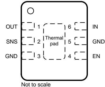
DRV Package (Fixed) 6-Pin WSON Top View
