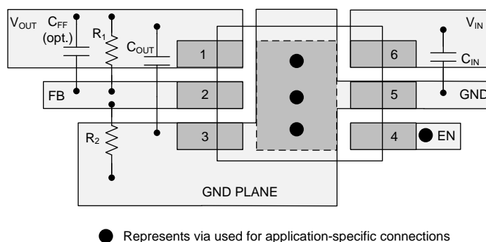
Figure 42. Layout Example for the Adjustable Version
