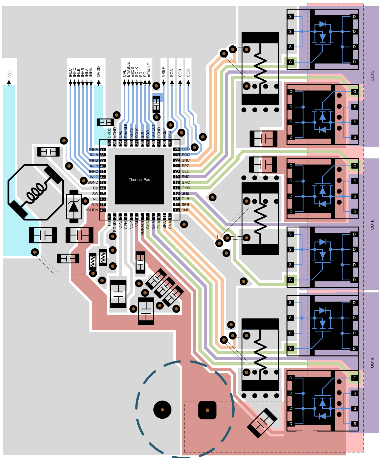
Figure 64. Layout Example
