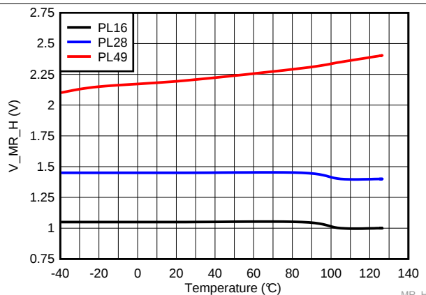
Figure 32. Manual Reset Logic High Voltage Threshold over Temperature for TPS3840PLXX
