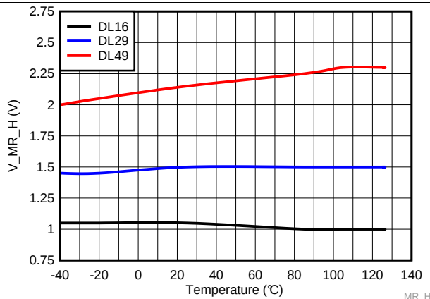
Figure 31. Manual Reset Logic High Voltage Threshold over Temperature for TPS3840DLXX
