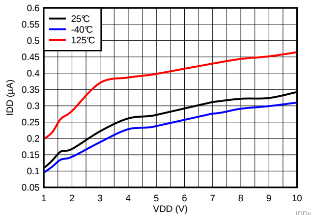
Figure 8. Supply Current vs Supply Voltage for TPS3840PH49
