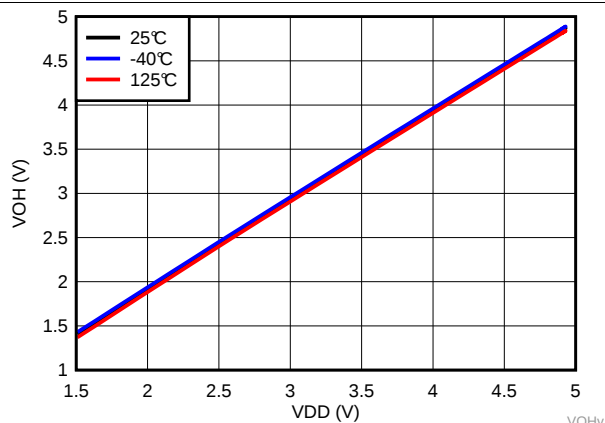
Figure 27. High Level Output Voltage over Temperature for TPS3840PH49
