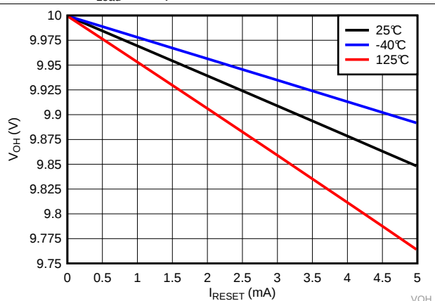
Figure 24. High Level Output Voltage vs I_{RESET} for TPS3840PL49
