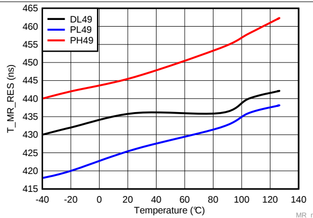
Figure 42. Propagation Time Delay from \overline{\text{MR}} Asserted to Reset over Temperature
