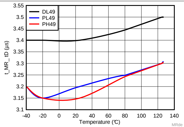
Figure 43. Propagation Time Delay from \overline{\text{MR}} Release to Deasserted Reset over Temperature
