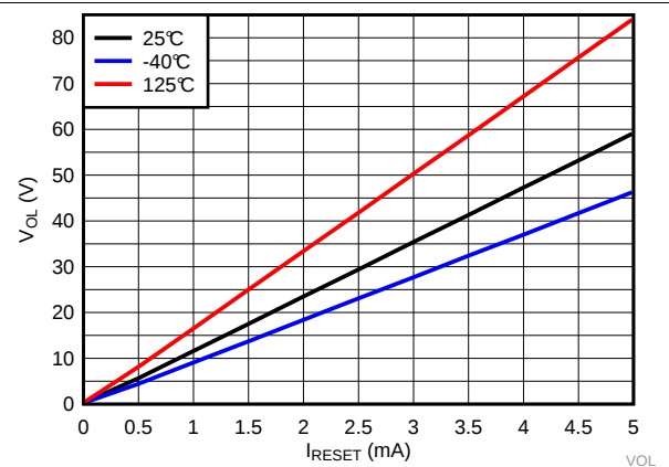
Figure 22. Low Level Output Voltage vs I_{RESET} for TPS3840PH49
