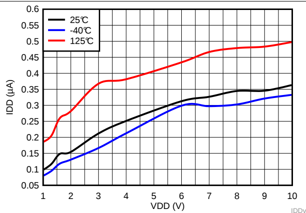
Figure 6. Supply Current vs Supply Voltage for TPS3840DL49
