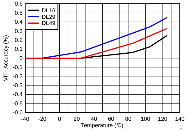
Figure 9. Negative-going Input Threshold Accuracy over Temperature for TPS3840DLXX
