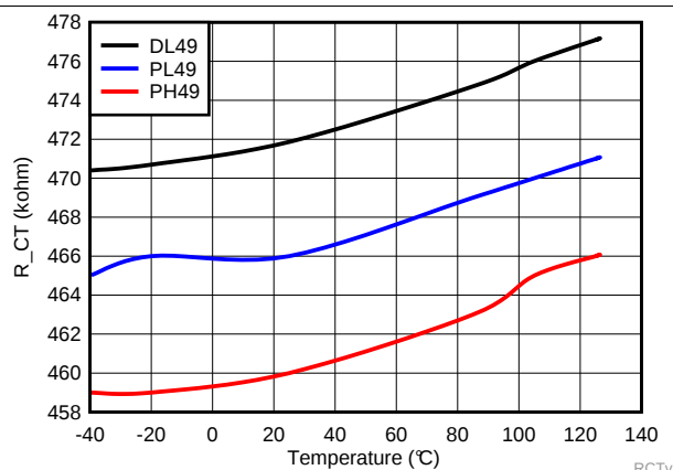
Figure 35. CT Pin Internal Resistance over Temperature
