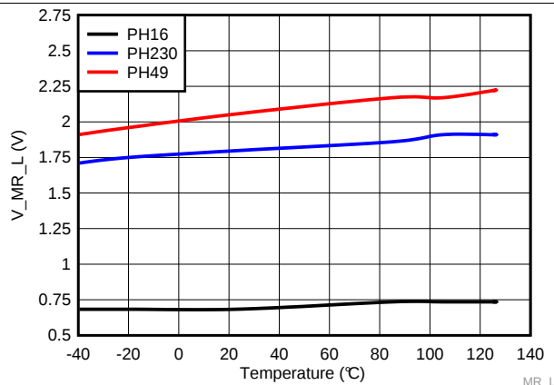
Figure 30. Manual Reset Logic Low Voltage Threshold over Temperature for TPS3840PHXX
