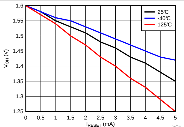
Figure 26. High Level Output Voltage vs I_{RESET} for TPS3840PH49
