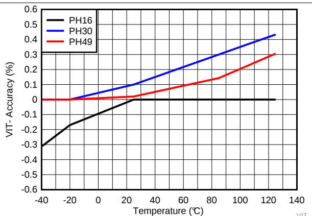
Figure 11. Negative-going Input Threshold Accuracy over Temperature for TPS3840PHXX
