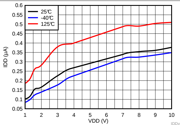
Figure 7. Supply Current vs Supply Voltage for TPS3840PL49
