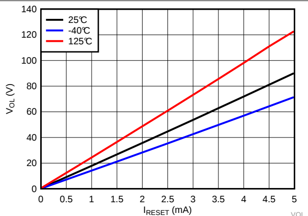
Figure 18. Low Level Output Voltage vs I_{RESET} for TPS3840DL49
