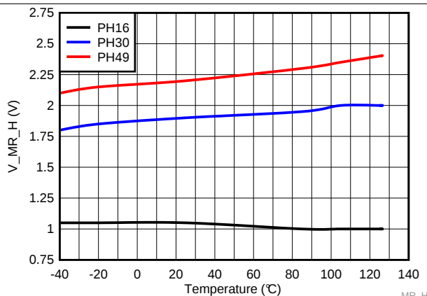
Figure 33. Manual Reset Logic High Voltage Threshold over Temperature for TPS3840PHXX
