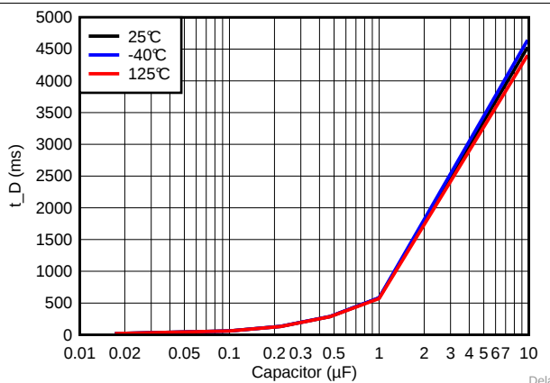
Figure 38. Reset Time Delay vs Capacitor Value (Data Taken with TPS3840PL16)
