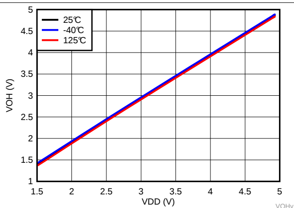
Figure 25. High Level Output Voltage over Temperature for TPS3840PL49
