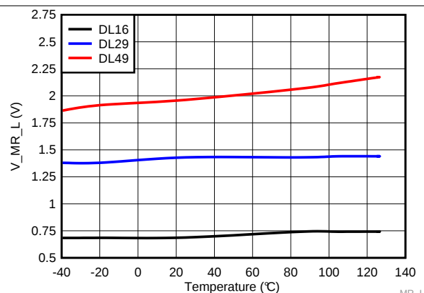
Figure 28. Manual Reset Logic Low Voltage Threshold over Temperature for TPS3840DLXX
