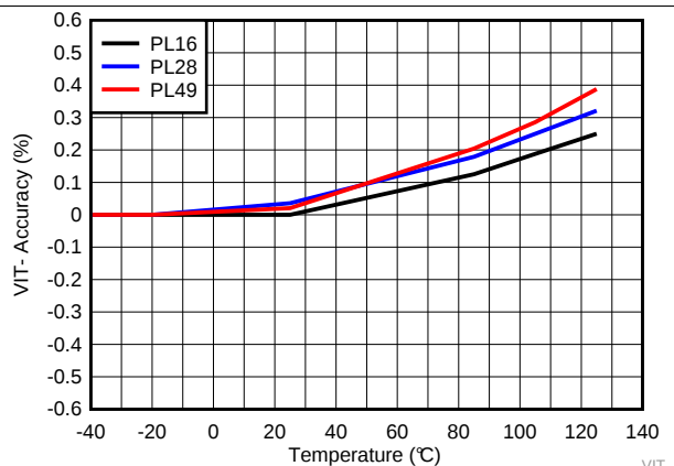
Figure 10. Negative-going Input Threshold Accuracy over Temperature for TPS3840PLXX
