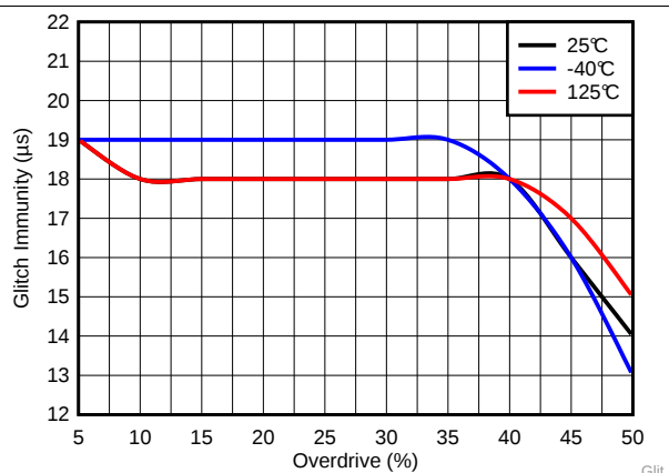
Figure 34. Glitch Immunity on V_{IT-} vs Overdrive (Data Taken with TPS3840PL28)
