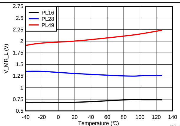
Figure 29. Manual Reset Logic Low Voltage Threshold over Temperature for TPS3840PLXX
