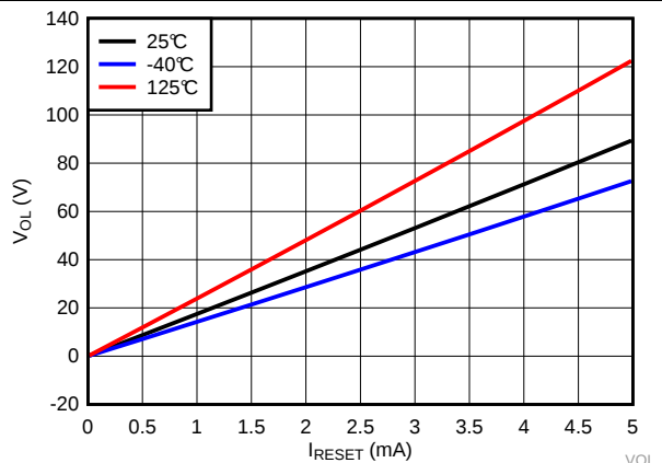
Figure 20. Low Level Output Voltage vs I_{RESET} for TPS3840PL49
