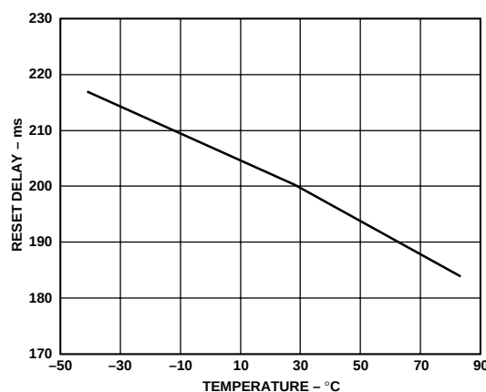
Figure 2. \overline{RESET} Timeout Delay vs. Temperature
