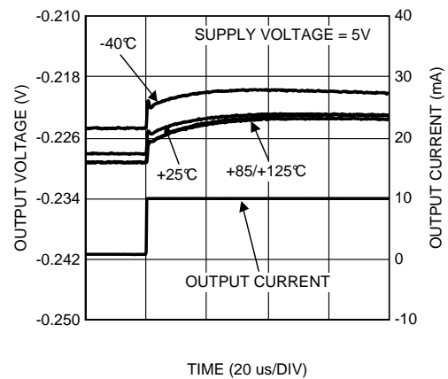
Figure 16. Transient Response
