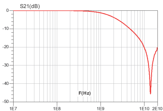
Figure 7. S21 attenuation
