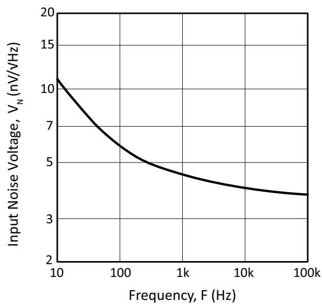
Figure 11: Input Noise
