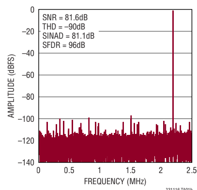
32k Point FFT f_{\text{SMP}} = 5\text{Mps} , f_{\text{IN}} = 2.2\text{MHz}
