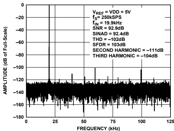
Figure 10. 20 kHz Fast Fourier Transform (FFT), V_{REF} = V_{DD} = 5\text{ V}
