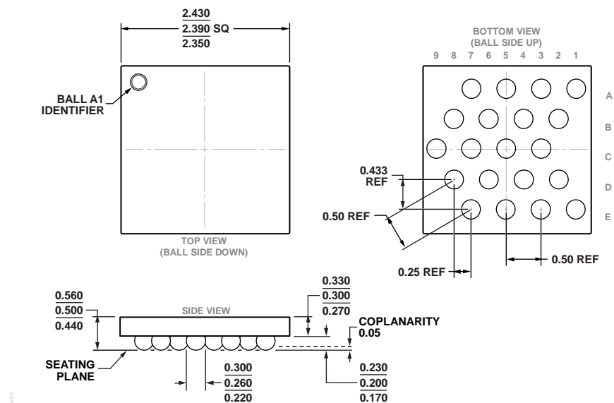
Figure 47. 20-Ball Wafer Level Chip Scale Package [WLCSP] (CB-20-12) Dimensions shown in millimeters
