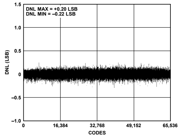
Figure 11. Differential Nonlinearity vs. Code, V_{REF} = V_{DD} = 5\text{ V}
