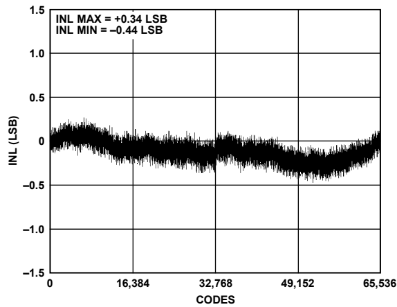
Figure 8. Integral Nonlinearity vs. Code, V_{REF} = V_{DD} = 5\text{ V}
