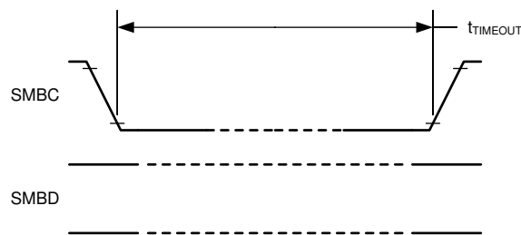
Figure 4. SMBus Timing Diagram
