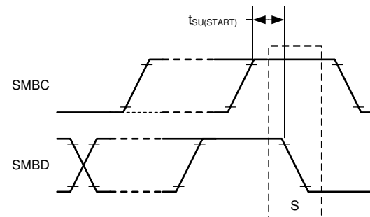
Figure 4. SMBus Timing Diagram
