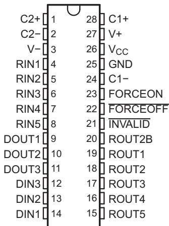
Pin Functions
