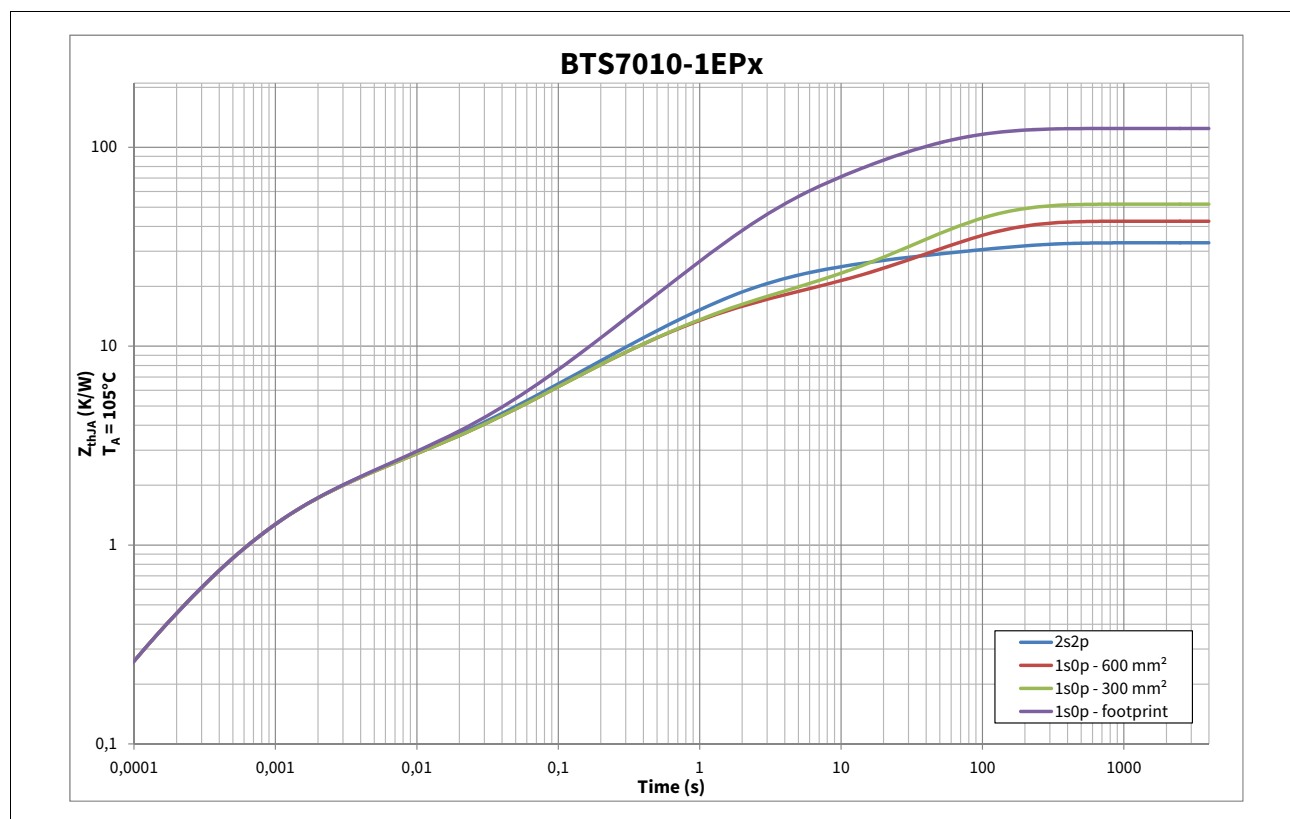
Figure 9 Typical Thermal Impedance. PCB setup according to Chapter 4.4.1
