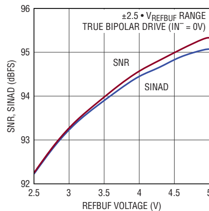
SNR, SINAD vs V_{REFBUF} , f_{IN} = 2\text{kHz}
