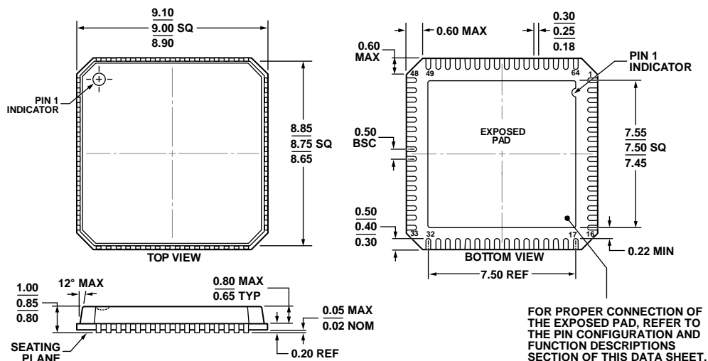
Figure 94. 64-Lead Lead Frame Chip Scale Package [LFCSP_VQ]
