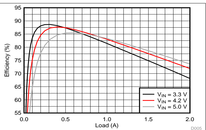
Figure 8. 0.6-V Output Efficiency
