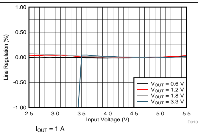
Figure 15. Line Regulation
