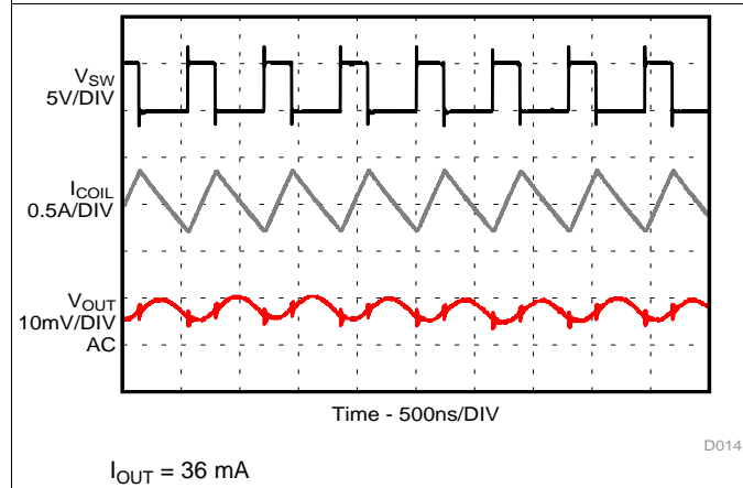
Figure 19. PWM Operation
