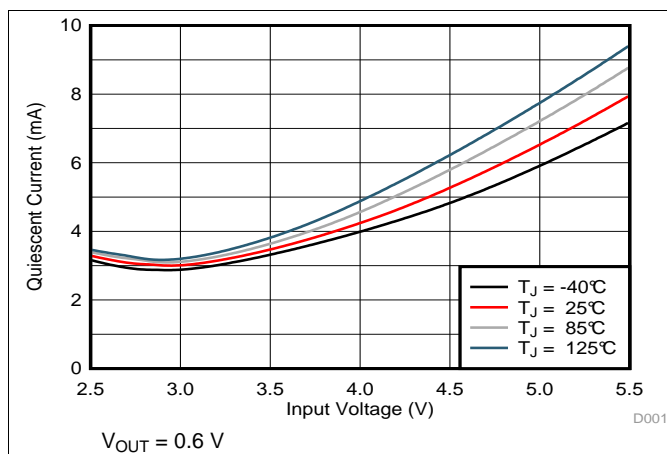
Figure 7. Quiescent Current
