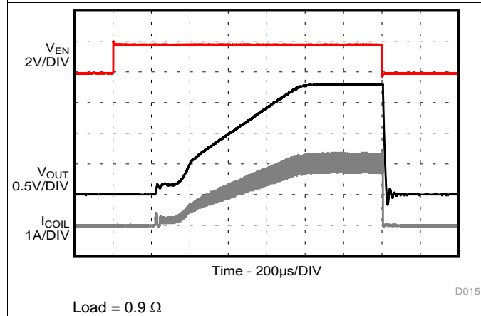
Figure 21. Startup and Shutdown with Load
