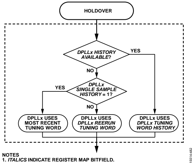
Figure 89. Holdover Flow Chart
