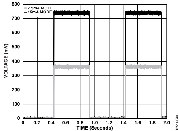
Figure 15. DC-Coupled, Single-Ended, 1 Hz Output Waveforms Using HCSSL 7.5 mA and 15 mA Mode Terminated 50\ \Omega to GND per Figure 45; Slew Rate: \sim 7\ \text{V/ns} for 15 mA Mode; \sim 3.5\ \text{V/ns} for 7.5 mA Mode
