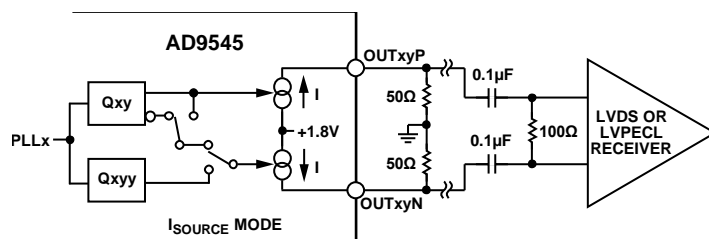
Figure 37. LVDS-Compatible Output Swing, AC-Coupled (375 mV (Differential) Across 100 \Omega Termination Resistor for I = 15 mA)
