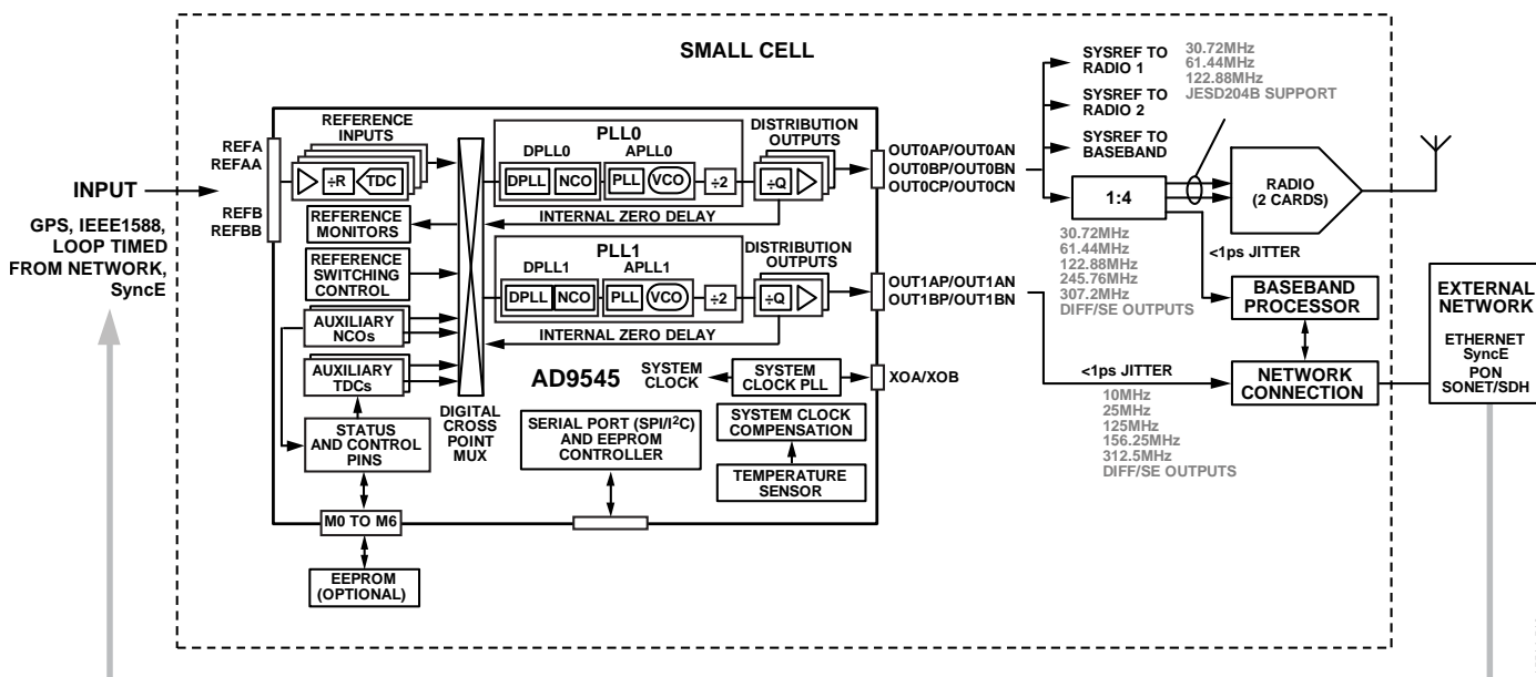
Figure 117. AD9545 Small Cell Application
