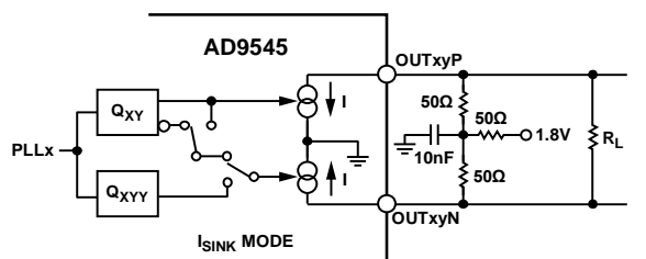
Figure 40. LVDS-Compatible Output, 1.24 V Common Mode, T Network ( I = 7.5 mA; I = 15 mA with Extra 100 \Omega Termination, R_L )
