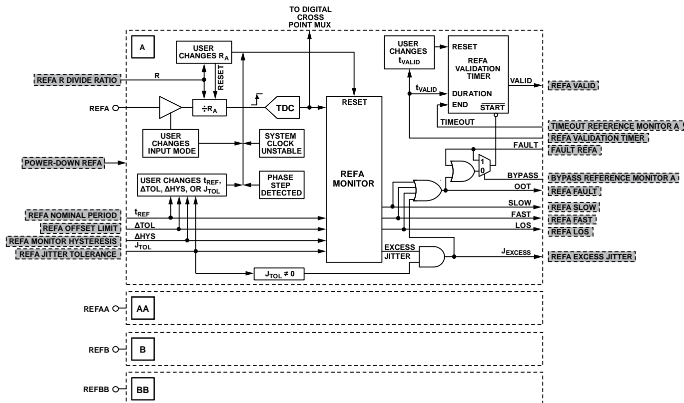
Figure 49. Reference Monitor
