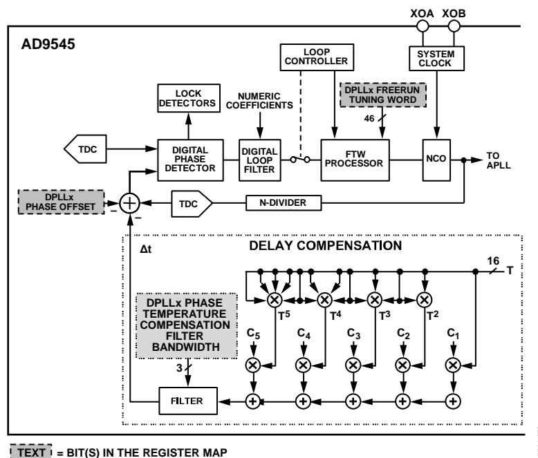
Figure 83. Delay Compensation
