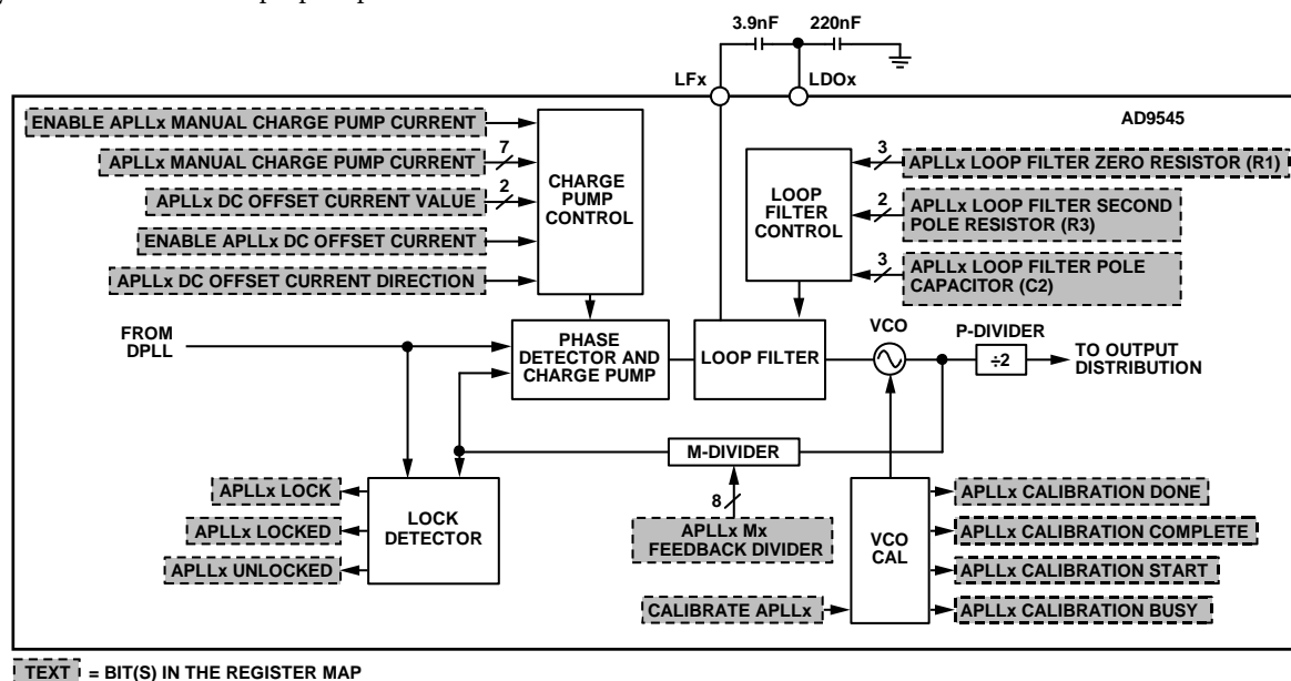
Figure 86. APLL Block Diagram
