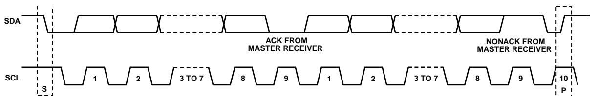
Figure 132. Data Transfer Process (Master Read Mode, 2-Byte Transfer), First Acknowledge From Slave
