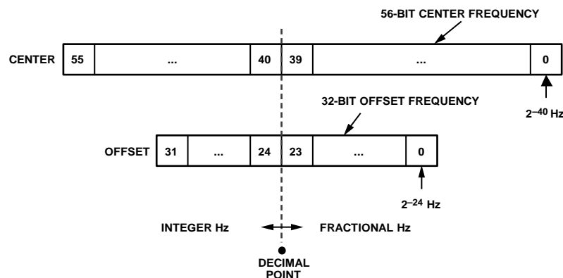
Figure 99. Auxiliary NCO Frequency Tuning
