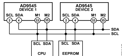
Figure 114. Level 2 Multidevice Configuration
