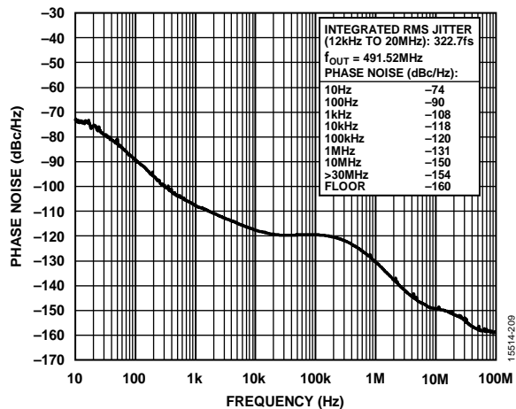
Figure 11. Absolute Phase Noise (PLL1, Configuration 3, HCSSL Mode, f_{REF} = 1\text{ Hz} , f_{OUT} = 491.52\text{ MHz} , f_{COMP} = 19.2\text{ MHz} TCXO, f_{OSC} = 52\text{ MHz} Crystal, 0.05 Hz DPLL BW)
