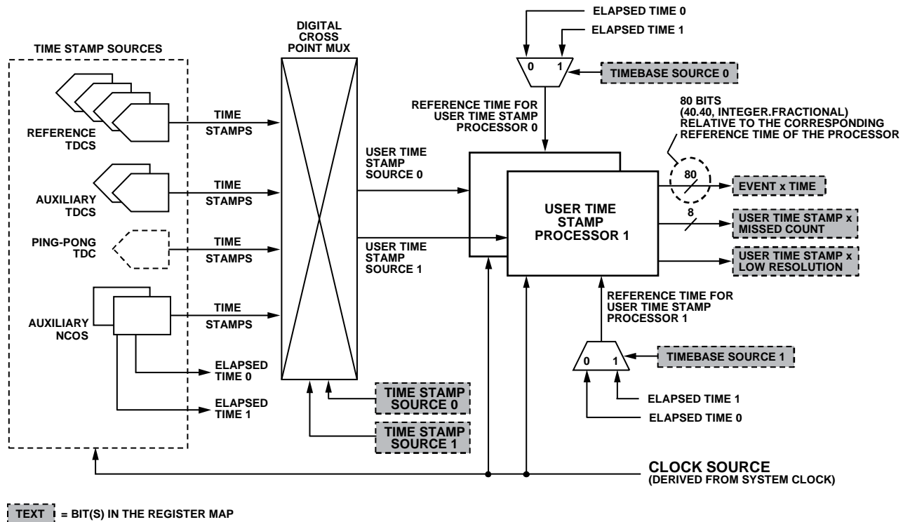
Figure 93. User Time Stamp Block Diagram
