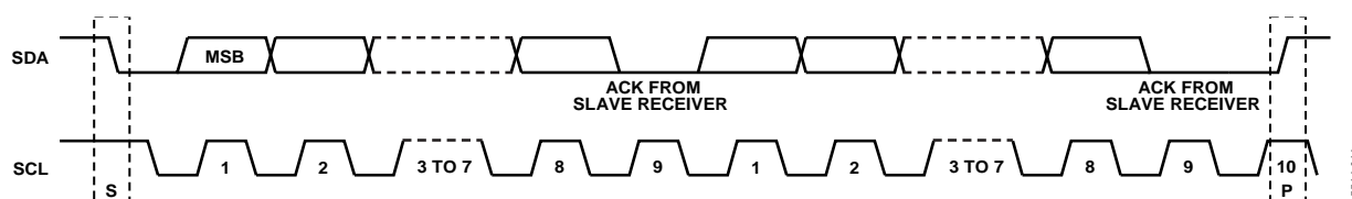
Figure 130. Acknowledge Bit
