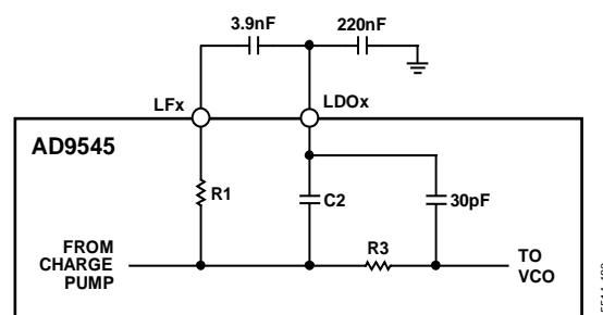
Figure 87. APLL Loop Filter
