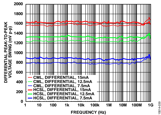
Figure 20. Differential Peak-to-Peak Voltage Swing vs. Frequency; HCSSL Drivers Terminated 50\ \Omega to GND per Figure 38; CML Drivers Terminated 50\ \Omega to 1.8 V per Figure 39
