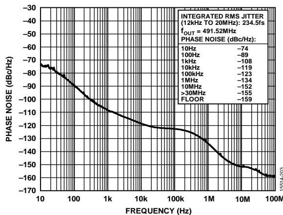
Figure 5. Absolute Phase Noise (PLL0, Configuration 3, HCSSL Mode, f_{REF} = 1\text{ Hz} , f_{OUT} = 491.52\text{ MHz} , f_{COMP} = 19.2\text{ MHz} TCXO, f_{OSC} = 52\text{ MHz} Crystal, 0.05 Hz DPLL BW)
