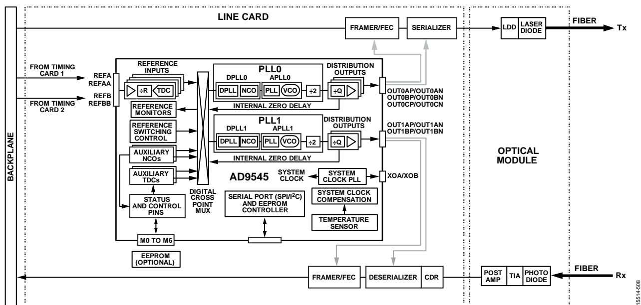
Figure 115. Optical Line Card Direct Timing Example
