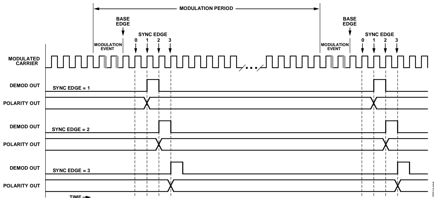
Figure 52. Demodulation Synchronization
