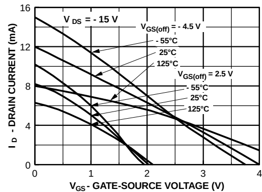
Transfer Characteristics
