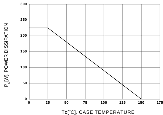
Power Derating
