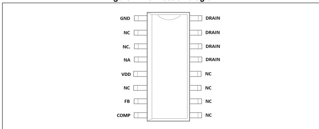
Figure 2. Connection diagram
