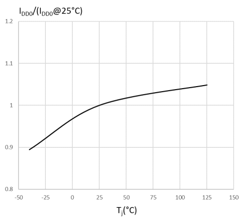
Figure 8. I_{DD0} vs. T_j
