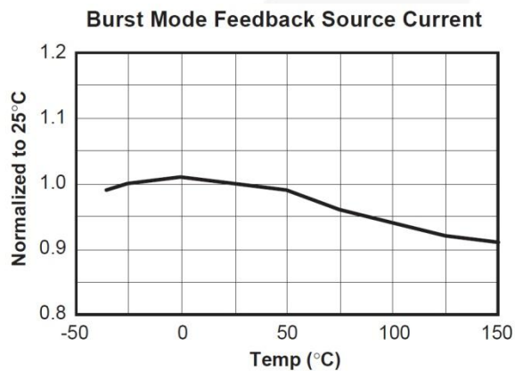
Figure 15. Burst Mode Feedback Source Current
