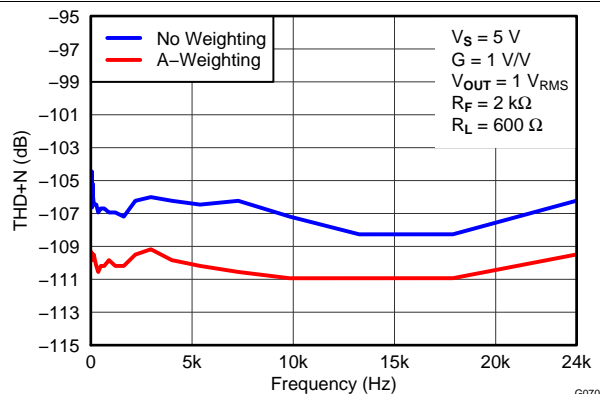
Figure 80. THD+N on Audio Analyzer, 10 Hz to 24 kHz
