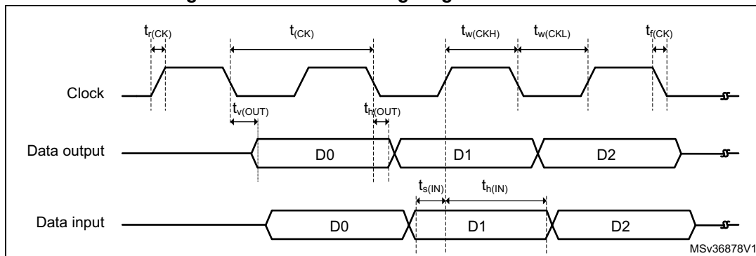
Figure 74. Quad-SPI timing diagram - SDR mode
