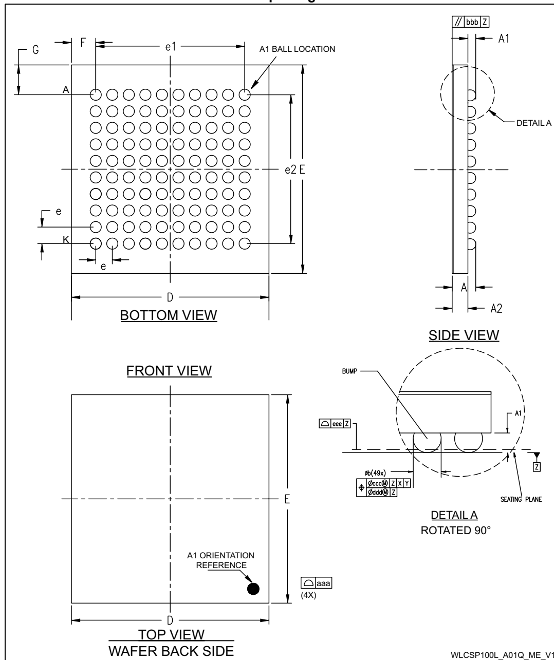
Figure 96. WLCSP100 – 100L, 4.166 x 4.628 mm 0.4 mm pitch wafer level chip scale package outline
